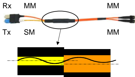
Figure 6: Mode conditioning
