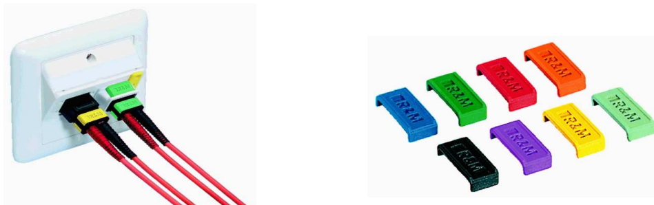
Figure 10: Security system. Left picture: colour coding for unequivocal plugging-in; plug-out protection preventing inadvertent and unauthorised disconnection. Right picture: colour coding clips – simply snapped onto the connectors.
